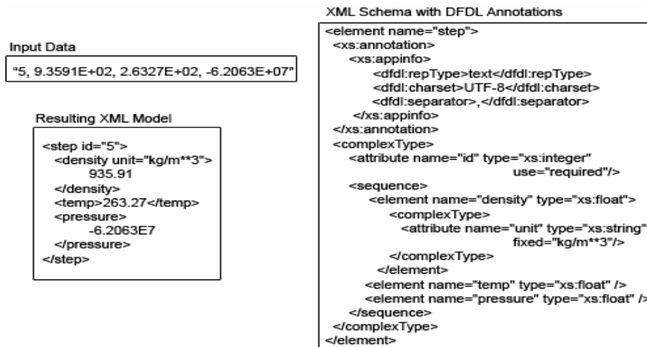
Fig. 1. Example of a DFDL schema with input data and results
